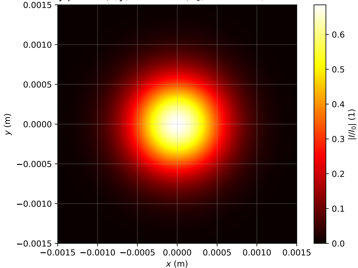
Intensity profile I(x, y, z = 1.672m)/I_0 , P_{in}=0.2P_{cr} , artificial time
